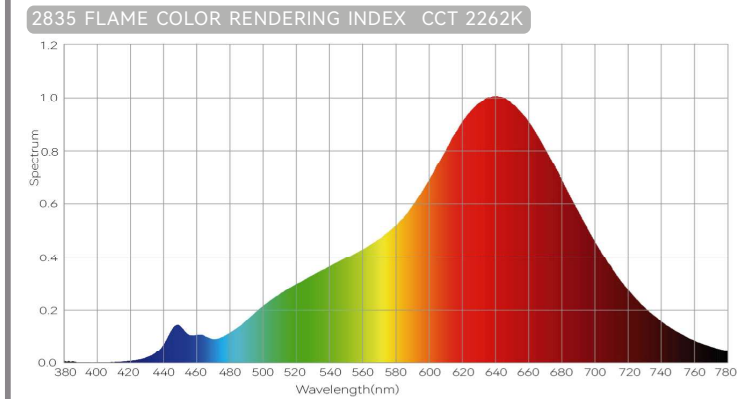
2835 FLAME COLOR SPECTRUM & WAVELENGTH CCT 2262K Ra=96.6
