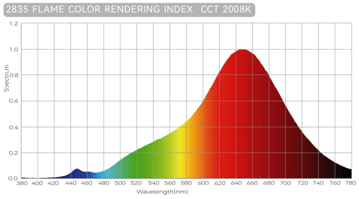
2835 FLAME COLOR SPECTRUM & WAVELENGTH CCT 2008K Ra=97.1
